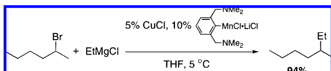
Scheme 196
