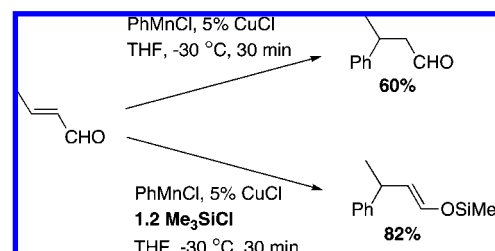
Scheme 133
