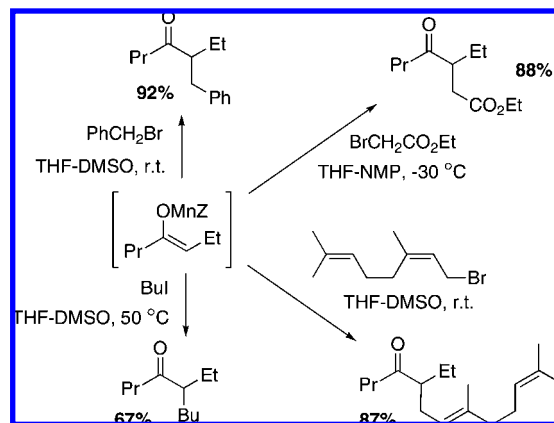
Scheme 146
