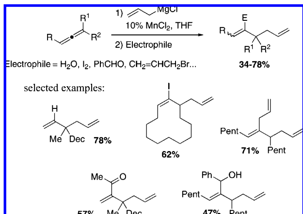
Scheme 233
