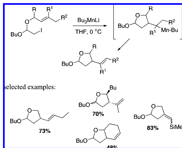
Scheme 244
