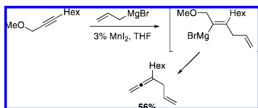
Scheme 224
