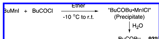
Scheme 79
