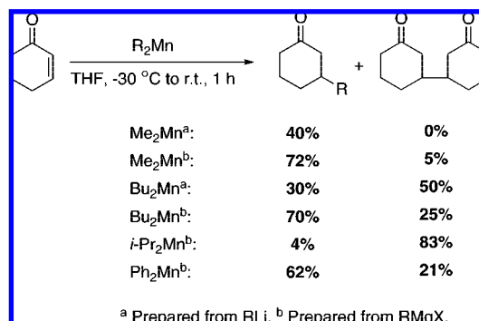
Scheme 108
