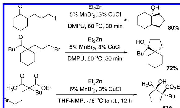
Scheme 240
