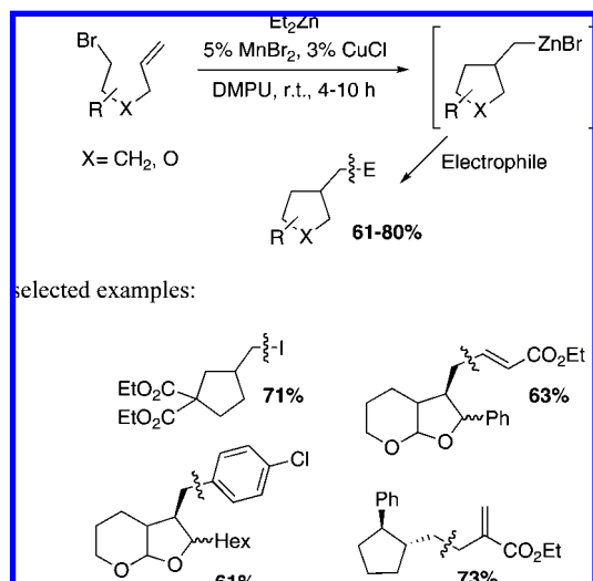
Scheme 239
