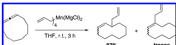
Scheme 232
