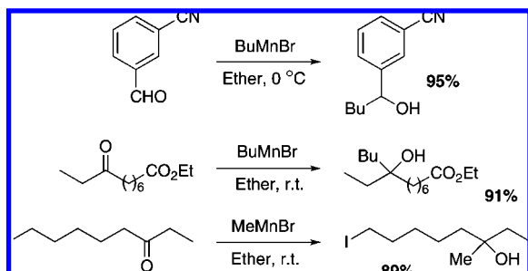
Scheme 57
