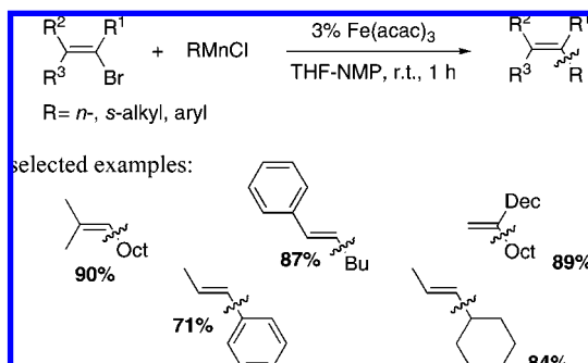
Scheme 183
