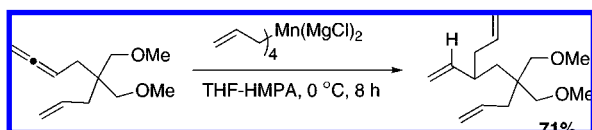
Scheme 234
