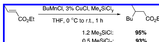
Scheme 128
