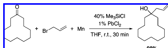
Scheme 29
