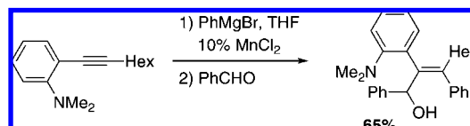
Scheme 229
