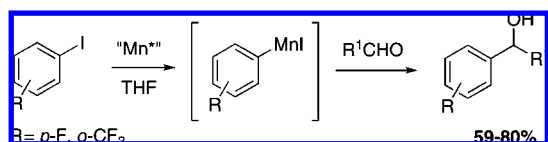
Scheme 42
