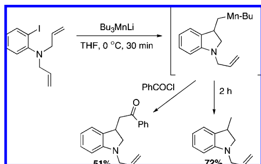
Scheme 240
