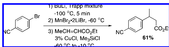
Scheme 131
