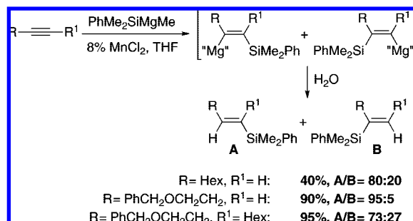
Scheme 219
