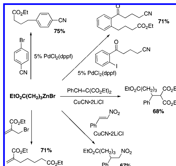
Figure 8. Mn/Cu-Catalyzed bromide–zinc exchange reaction.
