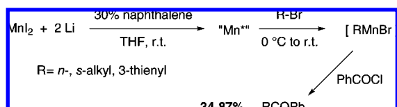
Scheme 32
