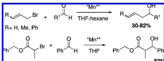
Scheme 41
