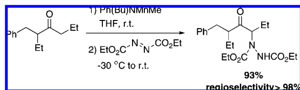
Scheme 152
