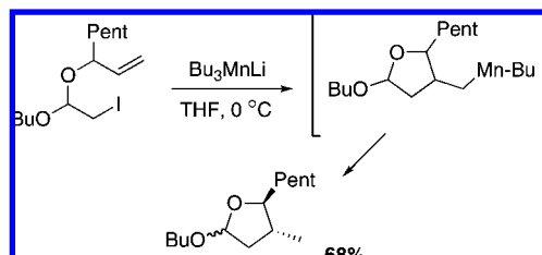
Scheme 243
