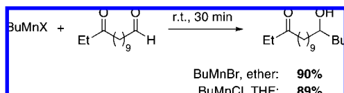
Scheme 56
