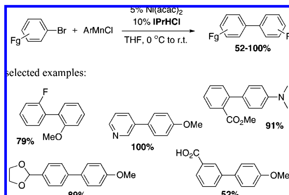
Scheme 180
