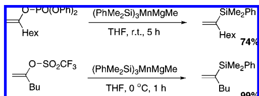
Scheme 201
