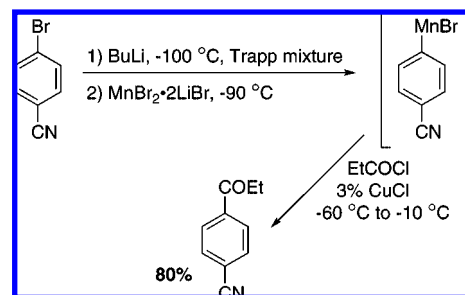
Scheme 19
