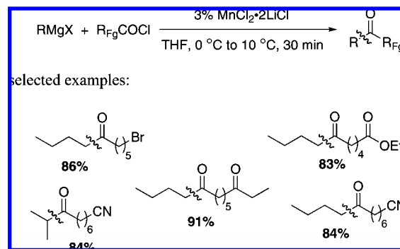
Scheme 96
