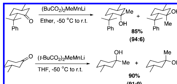
Scheme 65
