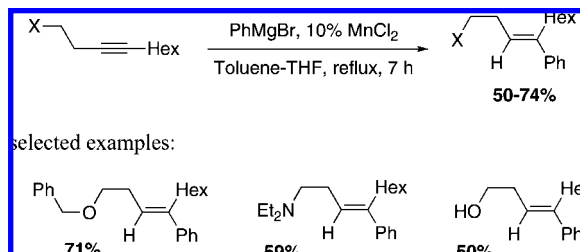
Scheme 228
