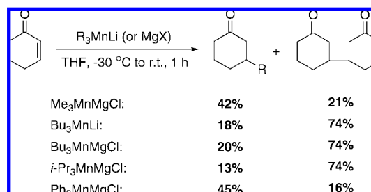
Scheme 108
