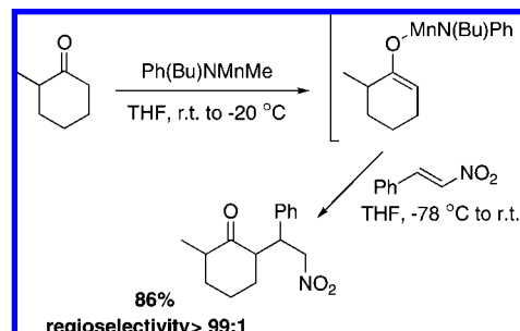
Scheme 151
