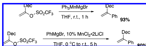
Scheme 201
