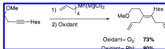
Scheme 226
