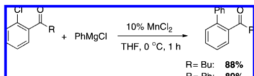
Scheme 172
