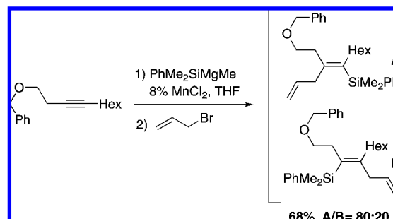
Scheme 219
