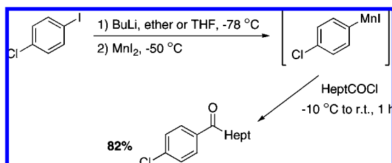
Scheme 17
