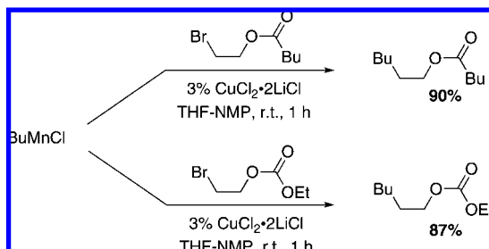
Scheme 194
