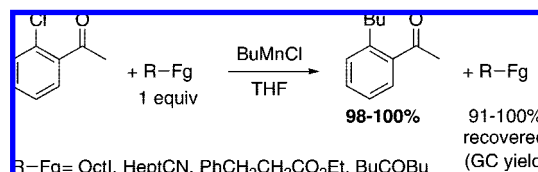
Scheme 214
