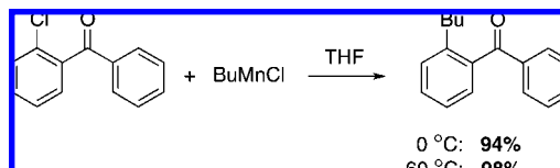
Scheme 211
