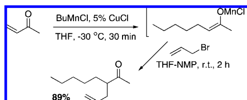
Scheme 160
