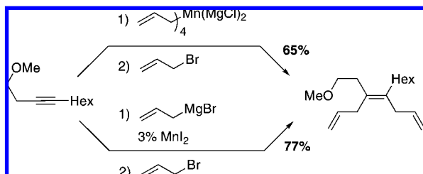
Scheme 222
