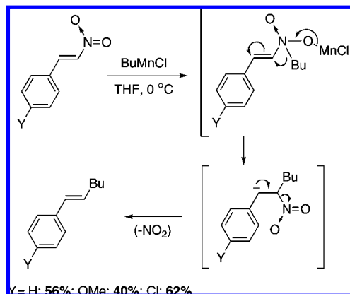
Scheme 122
