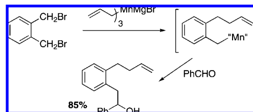
Scheme 210
