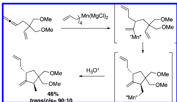
Scheme 234
