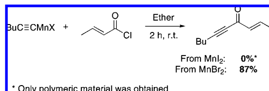
Scheme 82
