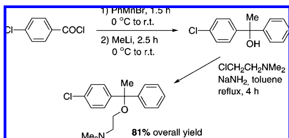
Scheme 104
