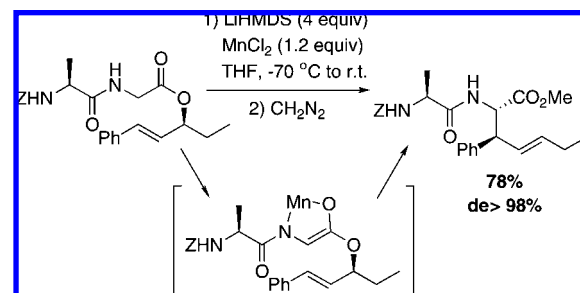
Scheme 160
