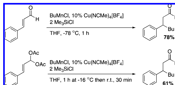
Scheme 134
