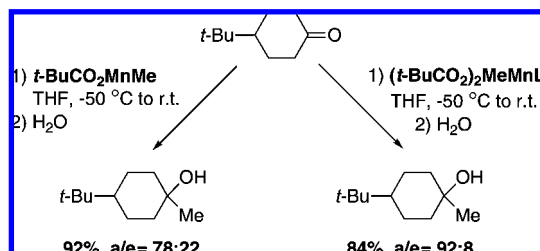
Scheme 64
