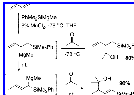
Scheme 229
