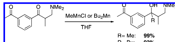
Scheme 61
