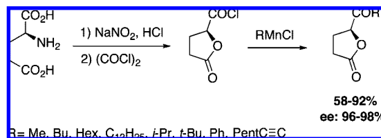
Scheme 106
