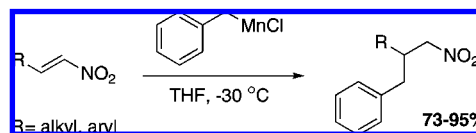
Scheme 121
