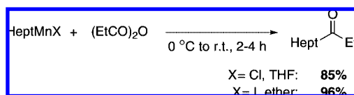
Scheme 91
