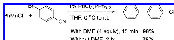
Scheme 176
