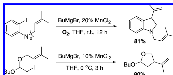
Scheme 244
