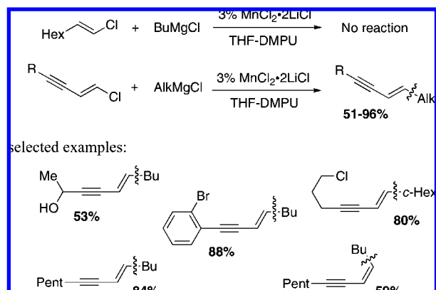
Scheme 176
