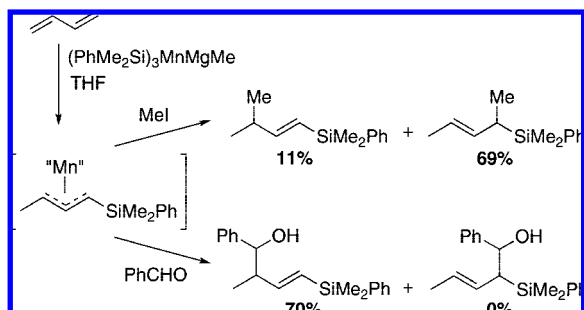
Scheme 231
