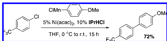
Scheme 182
