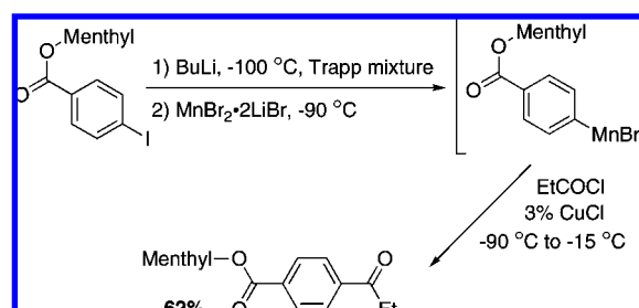
Scheme 20
