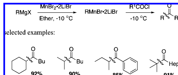
Scheme 81
