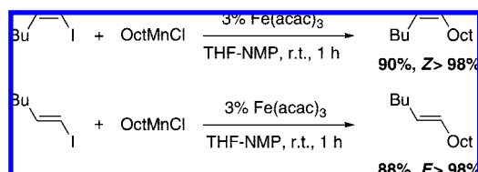
Scheme 185
