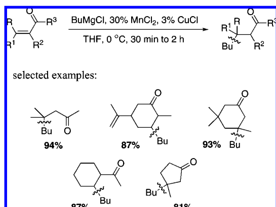
Scheme 126
