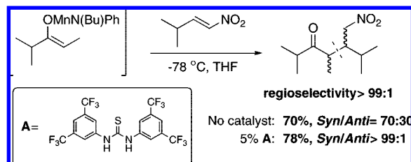
Scheme 152
