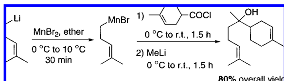
Scheme 103
