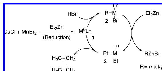
Figure 8. Mn/Cu-Catalyzed bromide–zinc exchange reaction.
