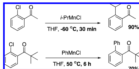
Scheme 212
