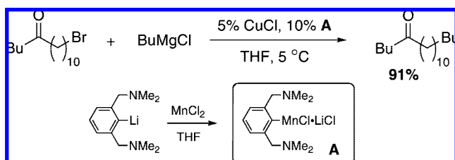
Scheme 196
