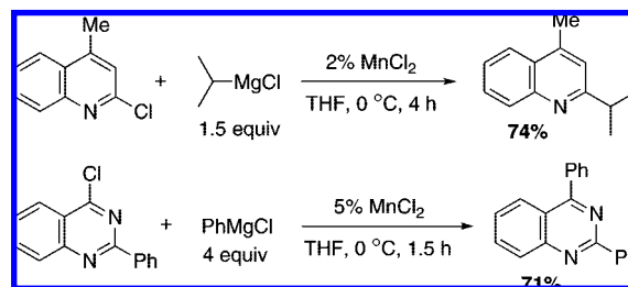
Scheme 175
