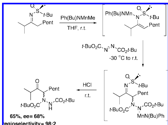
Scheme 154
