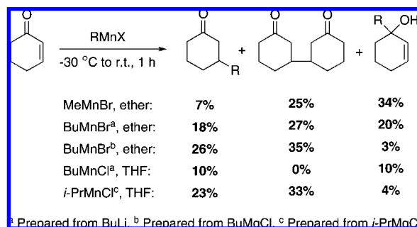
Scheme 107
