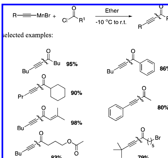
Scheme 83
