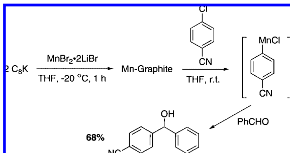
Scheme 32
