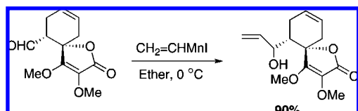
Scheme 57
