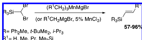
Scheme 207
