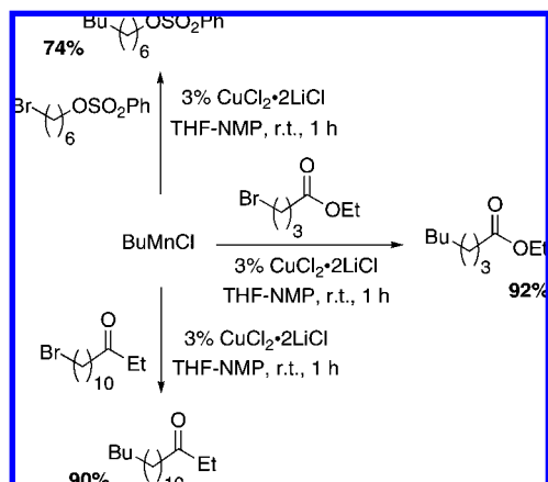
Scheme 192
