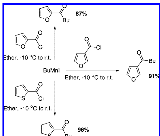
Scheme 77
