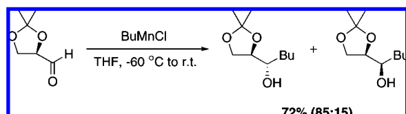
Scheme 62
