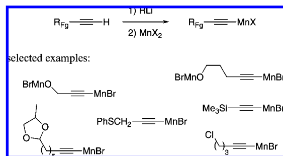
Scheme 21
