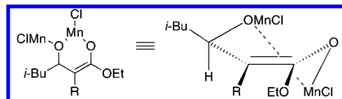
Figure 3. Mn-Mediated Reformatsky Reaction with \alpha,\alpha -Dichloroesters: Chelated Chair-Transition State.
