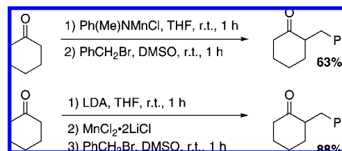
Scheme 157
