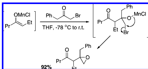
Scheme 147
