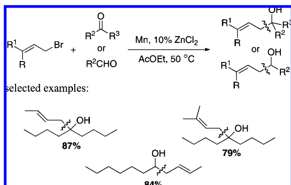
Scheme 26
