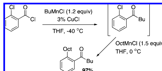
Scheme 214
