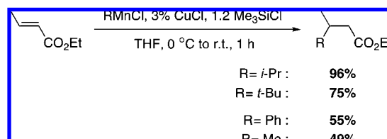
Scheme 129
