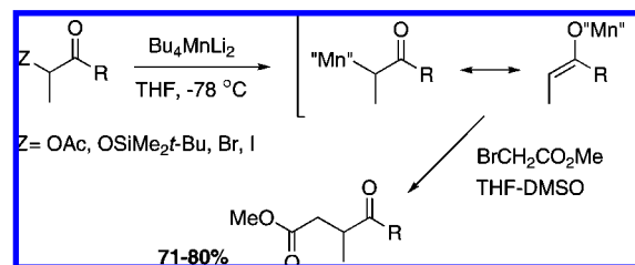
Scheme 45
