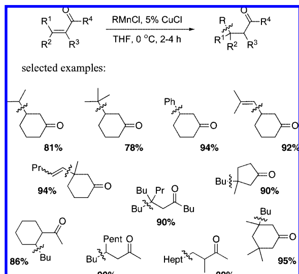
Scheme 125
