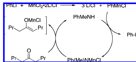
Figure 2. Amine-Catalyzed Deprotonation of Ketones by PhMnCl.
