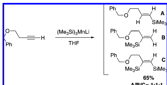
Scheme 217
