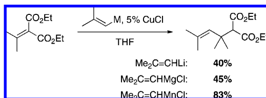
Scheme 117
