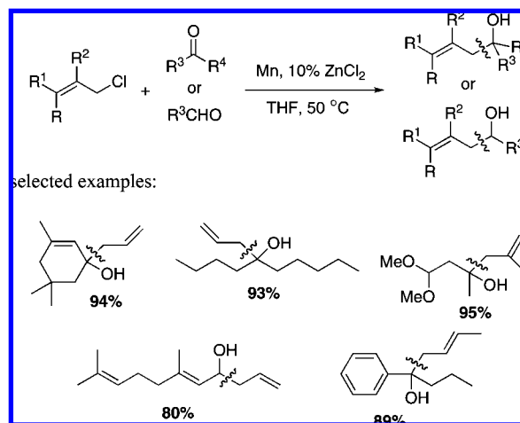
Scheme 28
