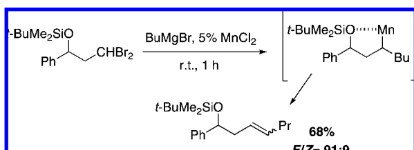
Scheme 208
