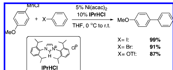
Scheme 180
