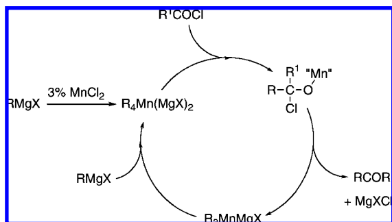
Figure 1. Mechanism of the Mn-catalyzed acylation of RMgX.
