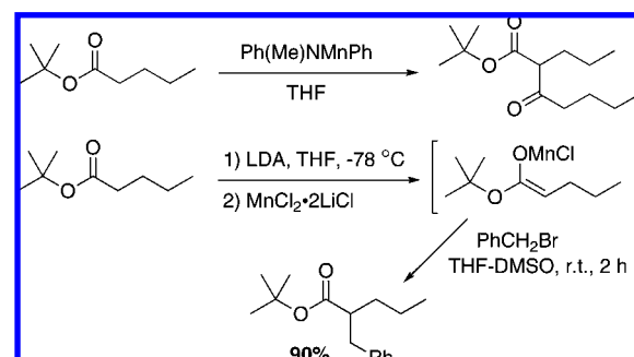
Scheme 159
