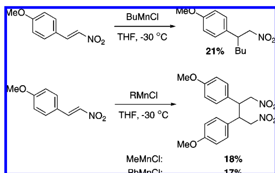
Scheme 119
