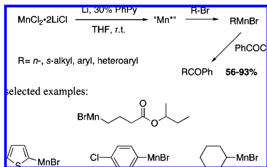
Scheme 38
