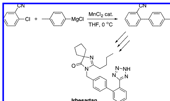
Scheme 174
