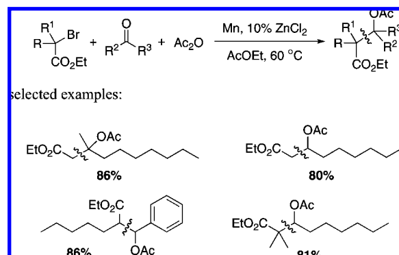
Scheme 29
