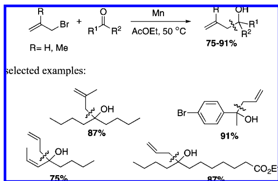
Scheme 26
